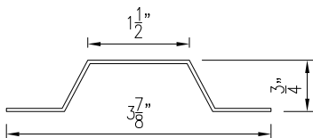
STIFFENER PROFILE
