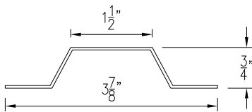
STIFFENER PROFILE
